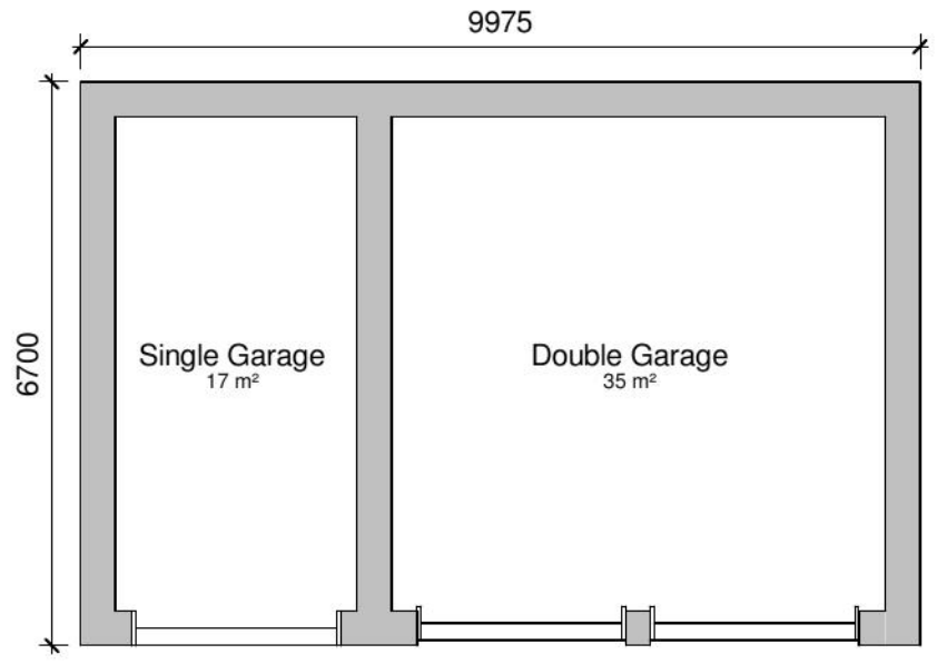
Garage 1 - Ground Floor 1 : 100
